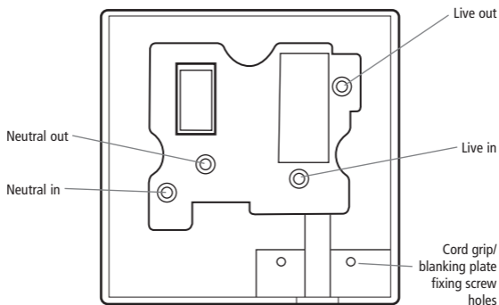
Fig. 2 TGBT4 Rear Connections
